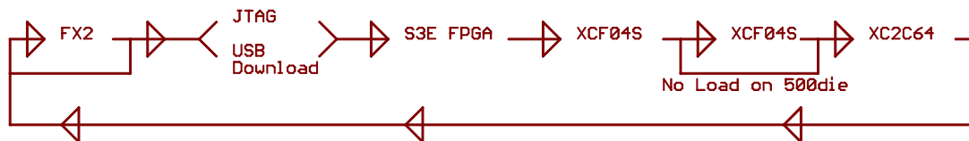
JTAG Scan Chain
