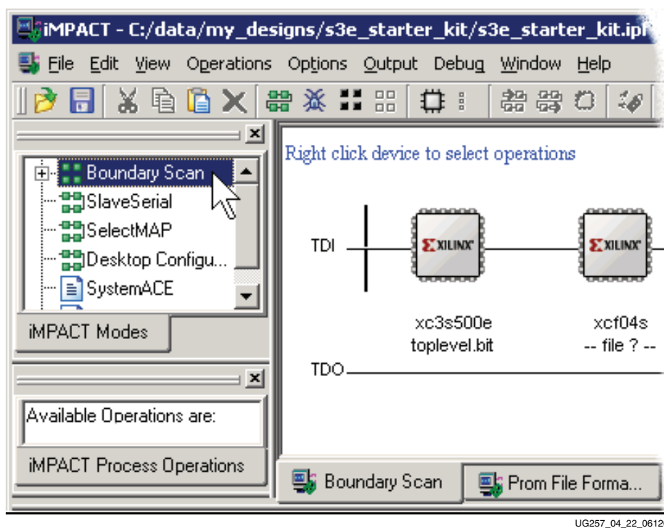
Figure 4-22: Switch to Boundary Scan Mode
