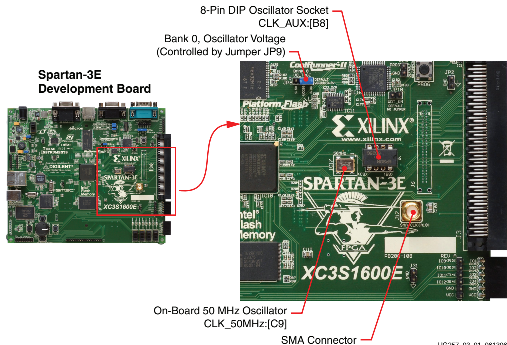
Figure 3-1: Available Clock Inputs
