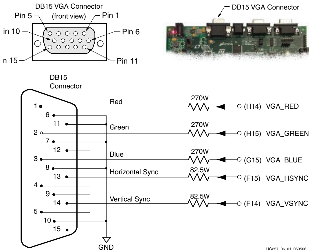
Figure 6-1: VGA Connections from Spartan-3E Starter Kit Board
