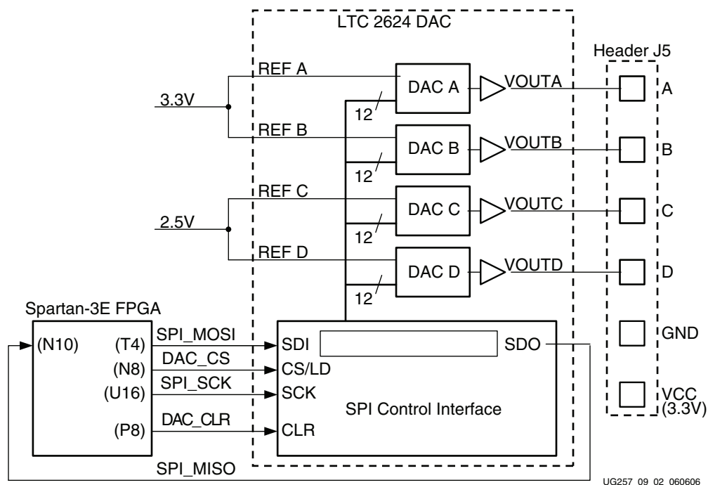
Figure 9-2: Digital-to-Analog Connection Schematics
