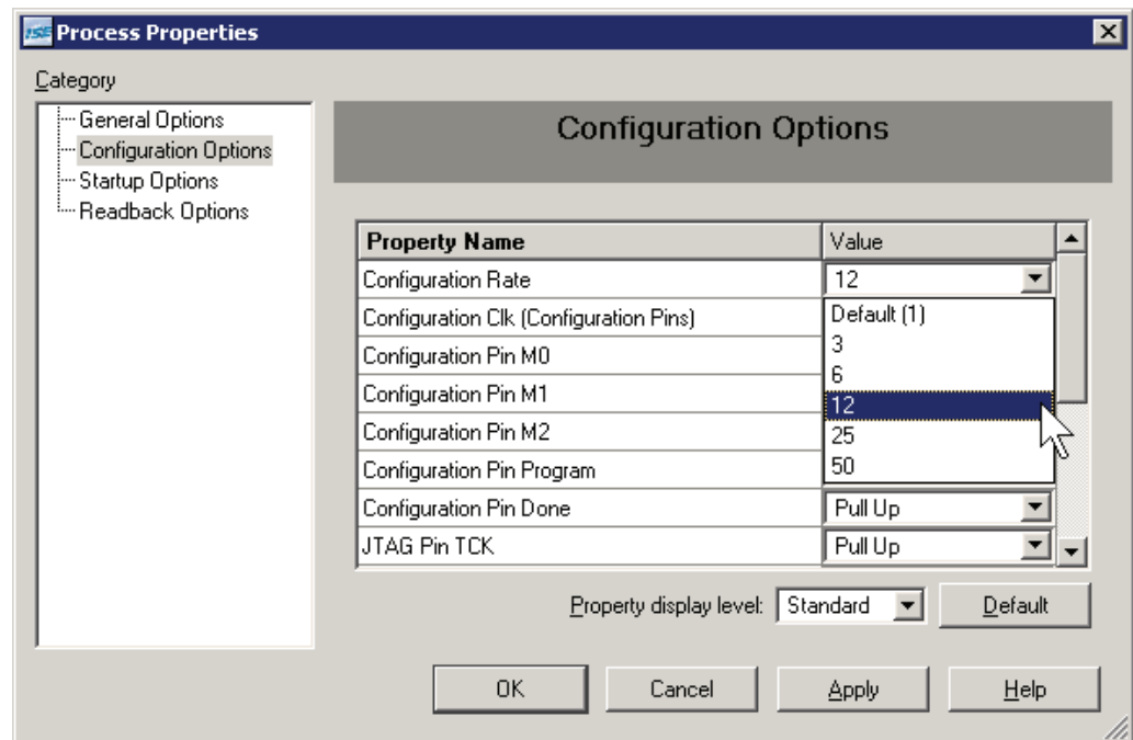
Figure 12-5: Set Configuration Rate to 12 MHz When Using the M25P16 SPI Flash
