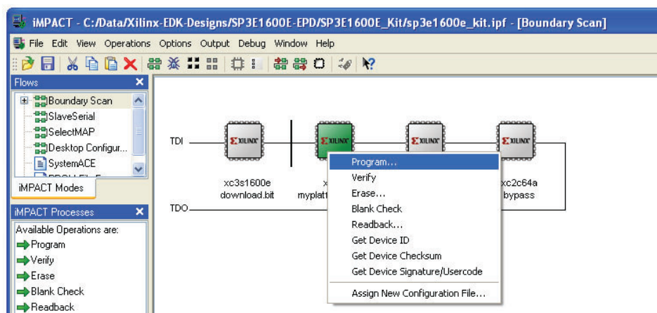
Figure 4-24: Program the XCF04S Platform Flash PROM
