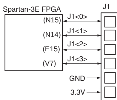
Figure 15-8: FPGA Connections to the J1 Accessory Header
