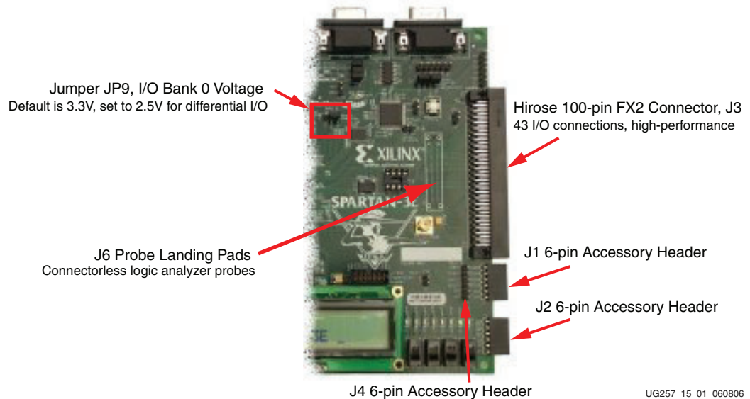
Figure 15-1: Expansion Headers
