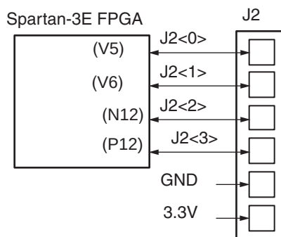
Figure 15-9: FPGA Connections to the J2 Accessory Header
