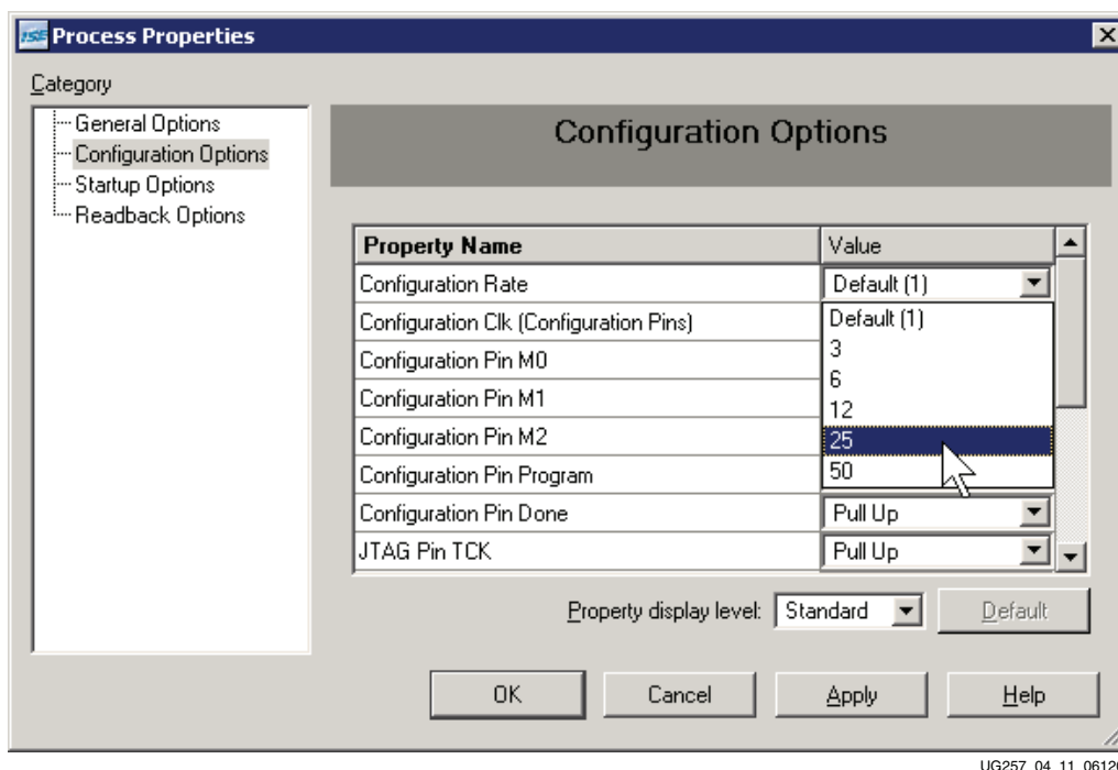
Figure 4-11: Set CCLK Configuration Rate under Configuration Options
