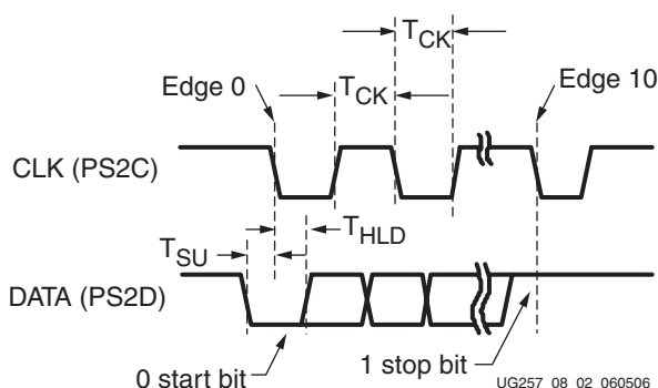
Figure 8-2: PS/2 Bus Timing Waveforms
