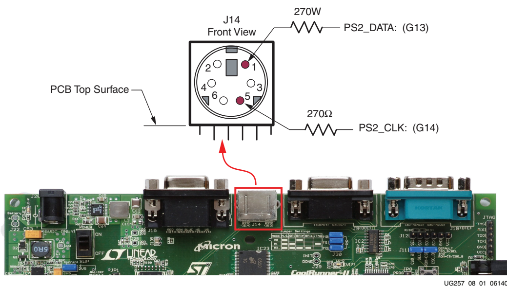
Figure 8-1: PS/2 Connector Location and Signals
