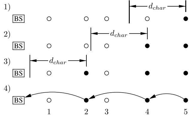
Fig. 1. Operation of MERR. In steps 1) to 3), the relays 4, 2, and BS are selected. The resulting path 5 \rightarrow 4 \rightarrow 2 \rightarrow BS approximates the optimal case and is used in step 4) to route data from sensor 5 to the base station.
