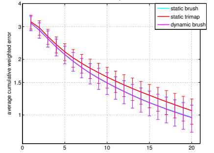
(c) GCA, \beta -scale w_\beta
